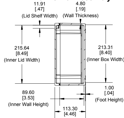
Top View of Box
