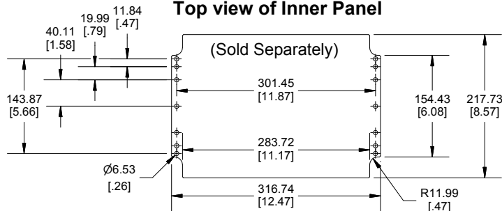
Top view of Inner Panel
