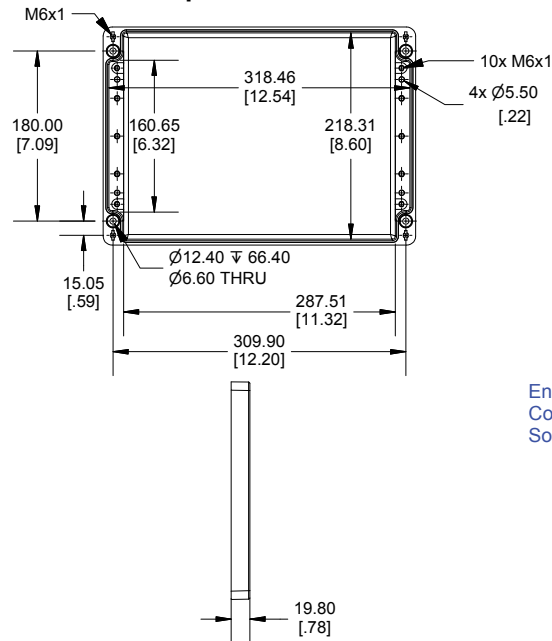
Top View of Box
