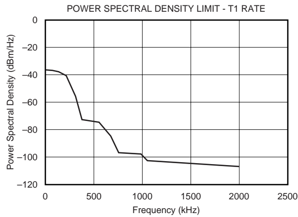
CURVE 1. Upper Bound of Power Spectral Density Measured at Output of HDSL Transformer.
