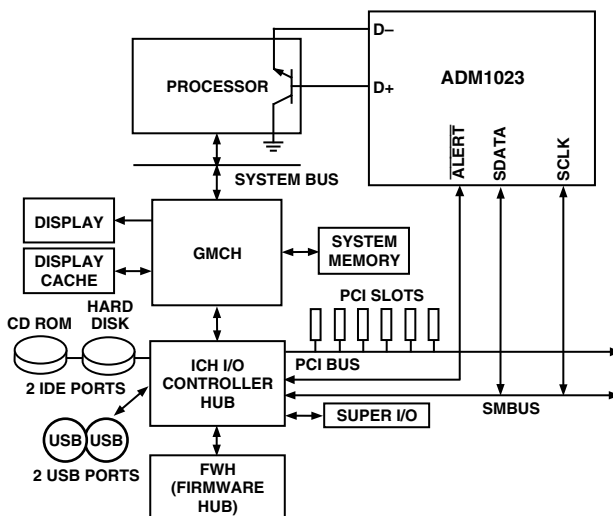
Figure 10. System Using ADM1023 and I/O Controller
