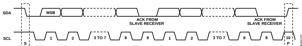
Figure 62. Acknowledge Bit
