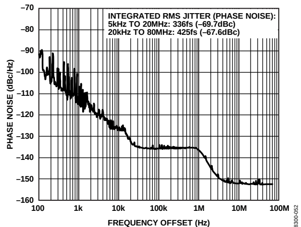
Figure 11. Absolute Phase Noise (Output Driver = LVPECL), f_{REF} = 8 kHz, f_0 = 155.52 MHz, LBW = 100 Hz, f_{SYSCLK} = 50 MHz (Crystal), PLL On
