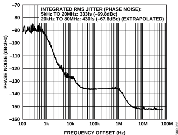
Figure 4. Absolute Phase Noise (Output Driver = LVPECL), f_{REF} = 19.44 MHz, f_0 = 155.52 MHz, LBW = 1 kHz, f_{SYSCLK} = 50 MHz (Crystal), PLL On
