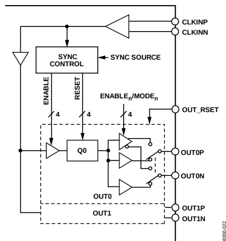
Figure 47. Clock Distribution
