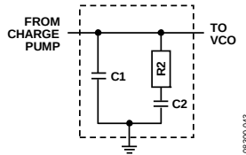
Figure 68. Second-Order Analog Loop Filter
