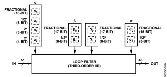
Figure 40. Third-Order Digital IIR Loop Filter
