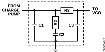
Figure 67. Third-Order Analog Loop Filter
