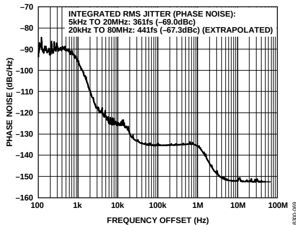
Figure 7. Absolute Phase Noise (Output Driver = LVPECL), f_{REF} = 19.44 MHz, f_0 = 155.52 MHz, LBW = 1 kHz, f_{SYSCLK} = 50 MHz, PLL On
