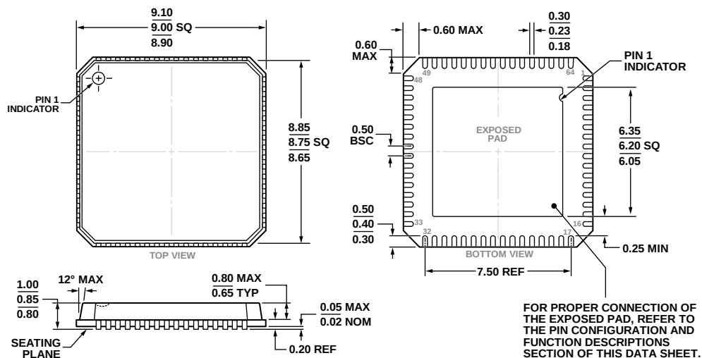
Figure 69. 64-Lead Lead Frame Chip Scale Package [LFCSP_VQ] 9 mm × 9 mm Body, Very Thin Quad (CP-64-4) Dimensions shown in millimeters
