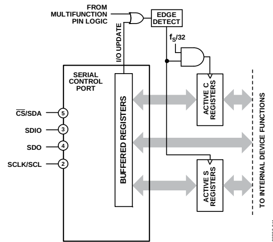
Figure 66. Buffered and Active Registers
