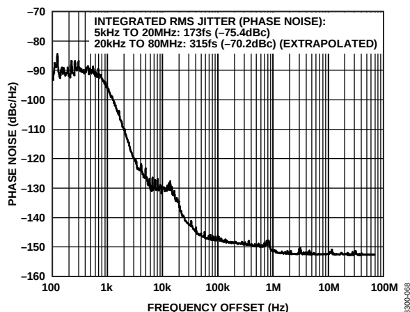
Figure 3. Absolute Phase Noise (Output Driver = LVPECL), f_{REF} = 19.44 MHz, f_0 = 155.52 MHz, LBW = 1 kHz, f_{SYSCLK} = 1 GHz, PLL Off
