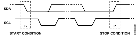
Figure 61. Start and Stop Condition
