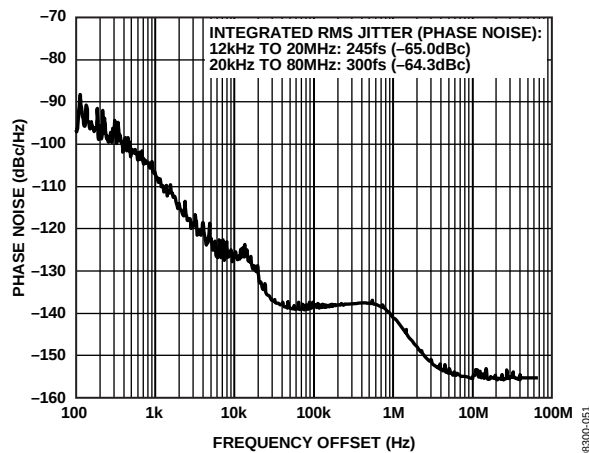
Figure 8. Absolute Phase Noise (Output Driver = LVPECL), f_{REF} = 19.44 MHz, f_0 = 155.52 MHz, LBW = 1 kHz, f_{SYSCLK} = 50 MHz (Crystal), PLL On with 2x Frequency Multiplier, I_{CP} = 375 \mu A, LF = External (350 kHz)
