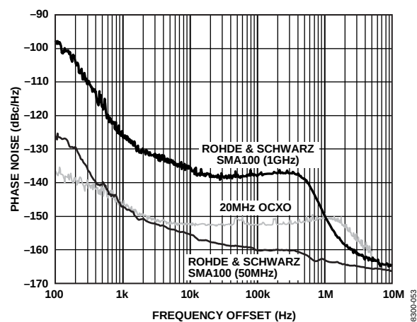
Figure 9. Phase Noise of SYSCLK Input Sources
