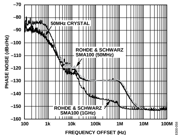
Figure 10. Absolute Phase Noise Comparison of SYSCLK Input Options (Output Driver = LVPECL), f_{REF} = 19.44 MHz, f_0 = 311.04 MHz, LBW = 1 kHz
