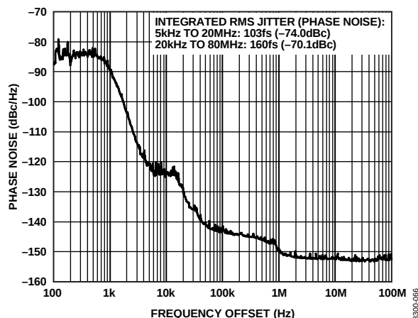
Figure 5. Absolute Phase Noise (Output Driver = LVPECL), f_{REF} = 19.44 MHz, f_0 = 311.04 MHz, LBW = 1 kHz, f_{SYSCLK} = 1 GHz, PLL Off
