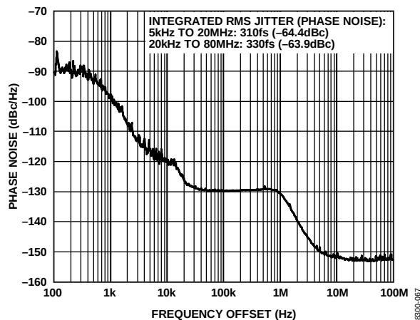
Figure 6. Absolute Phase Noise (Output Driver = LVPECL), f_{REF} = 19.44 MHz, f_0 = 311.04 MHz, LBW = 1 kHz, f_{SYSCLK} = 50 MHz (Crystal), PLL On
