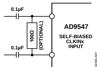
Figure 30. CLKINx Input
