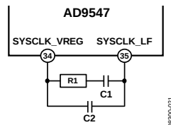
Figure 46. External Loop Filter Schematic
