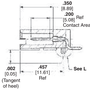
Section K-K
