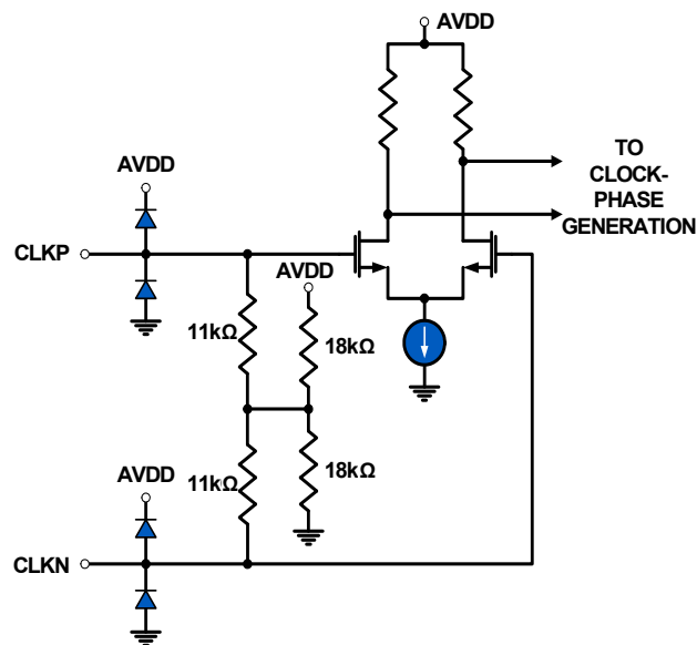
FIGURE 45. CLOCK INPUTS
