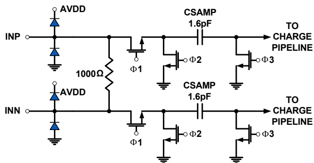
FIGURE 44. ANALOG INPUTS
