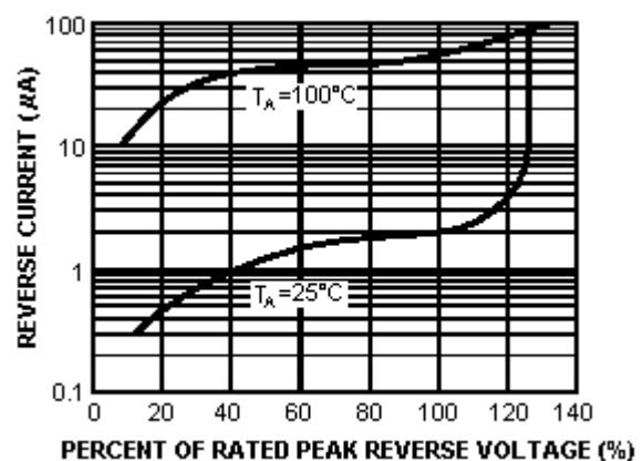
Reverse Characteristics
