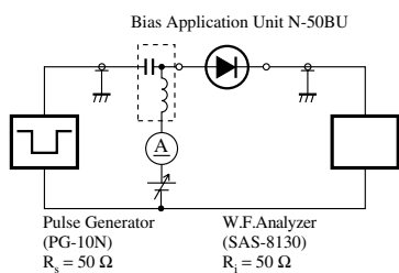
t_n measuring circuit
