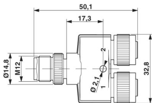
M12 Y distributor
