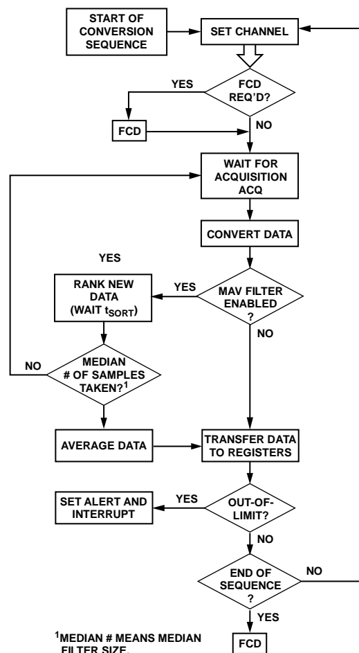
Figure 34. Conversion Sequence
