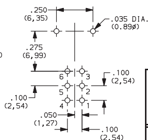
PC MOUNTING
