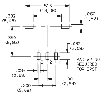
PC MOUNTING
