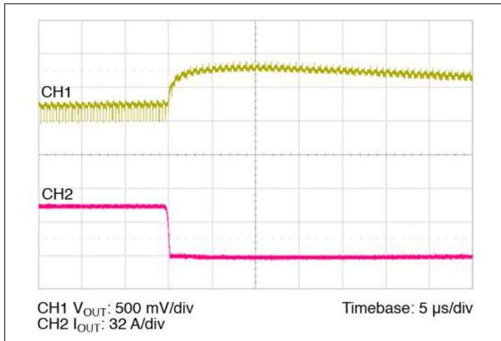
Figure 13 — 50 A–0 A transient response: C_{IN} = 100 \mu F , no external C_{OUT}
