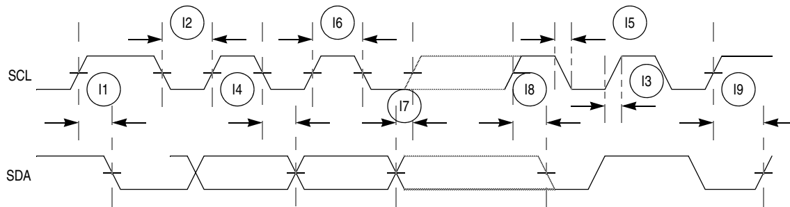
Figure 7. I²C Input/Output Timings
