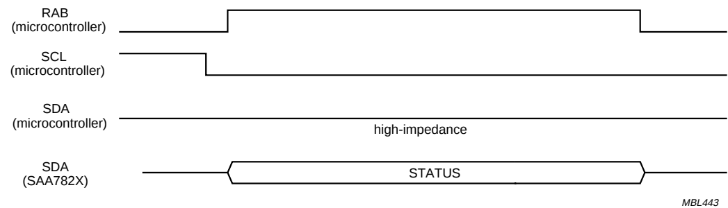
Fig.27 Microcontroller read protocol for decoder status on SDA.
