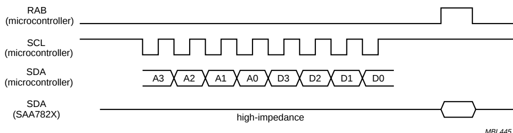
Fig.25 Microcontroller write protocol for registers 0 to F.
