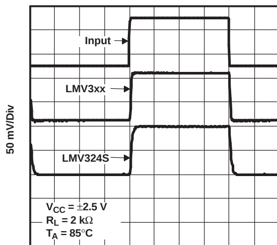
1 \mu\text{s/Div} Figure 31.
