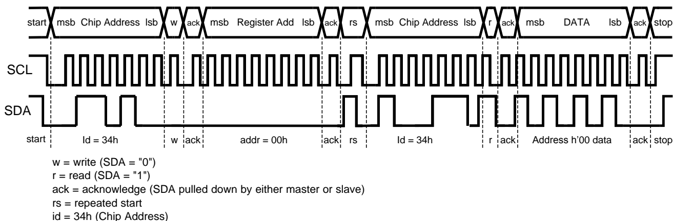
Figure 22. Read Cycle
