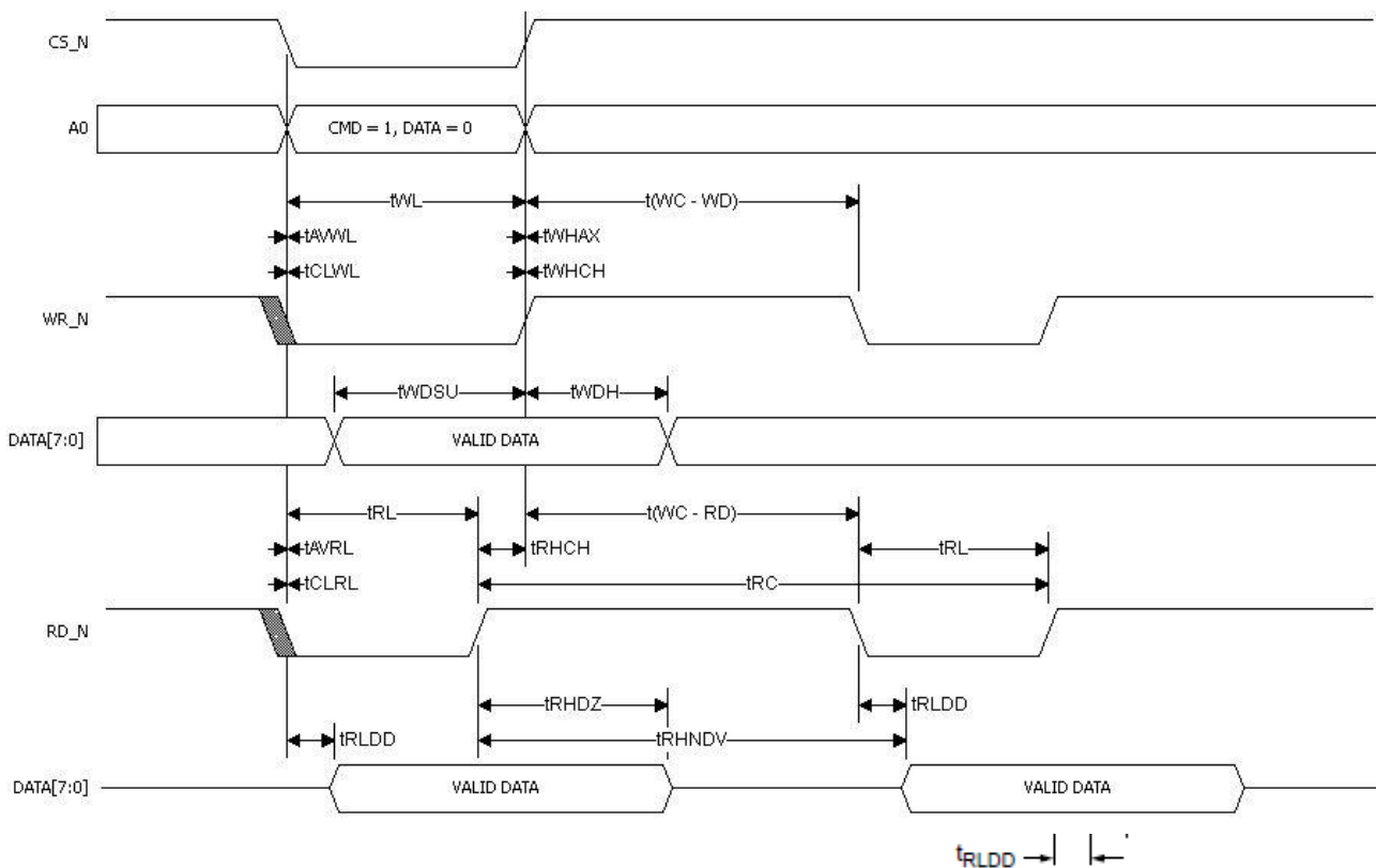
Figure 8-2 Parallel interface timing
