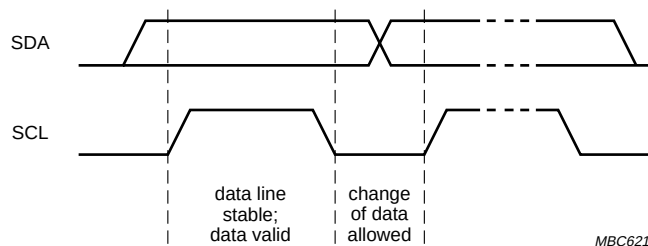
Fig.9 Bit transfer.
