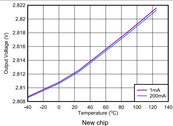
Figure 5-4. TPS793 Output Voltage vs Junction Temperature
