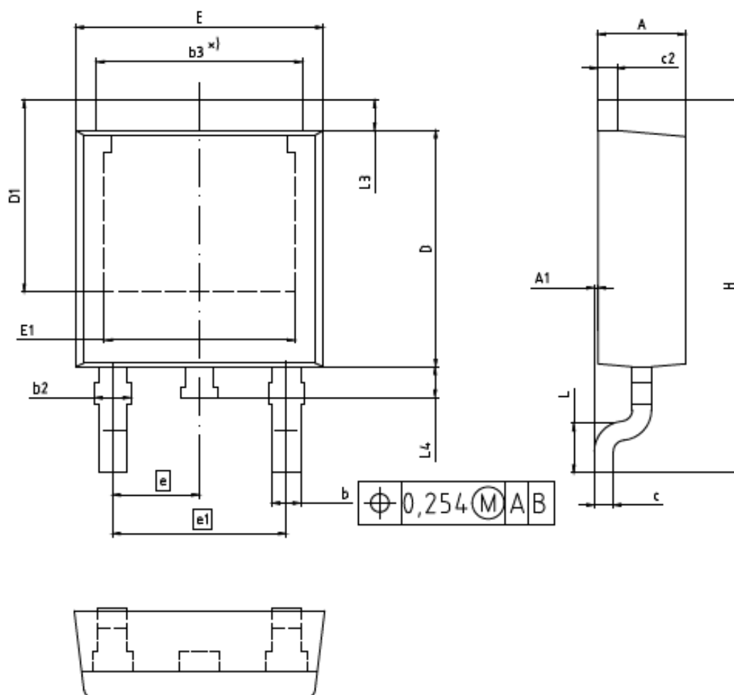
Package Drawing PG-T0252-3
