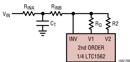
Figure 9. Lowpass “T” Input Circuit
