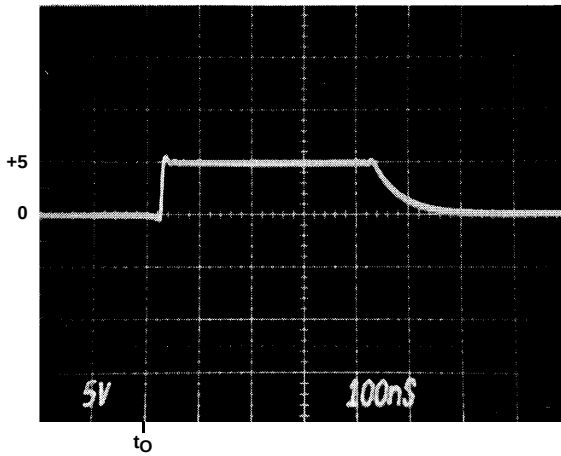
FIGURE 2C. V_{IN} = +5V
