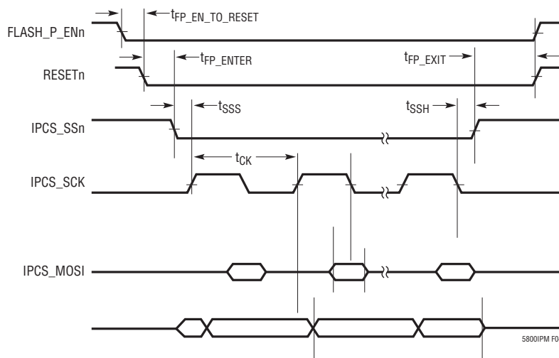
Figure 4. Flash Programming Interface Timing
