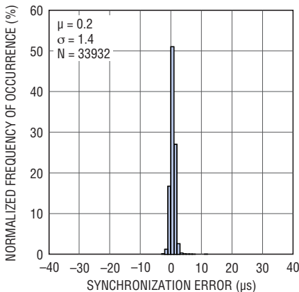
TIME n Synchronization Error 1 Packet/s Publishing Rate, 1 Hop, 8°C/Min
