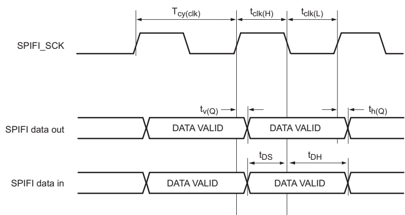
Fig 41. SPIFI timing
