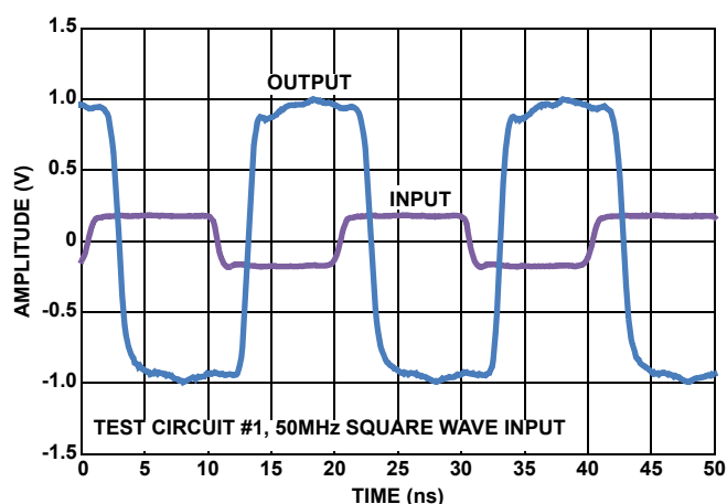
FIGURE 21. LARGE SIGNAL STEP RESPONSE
