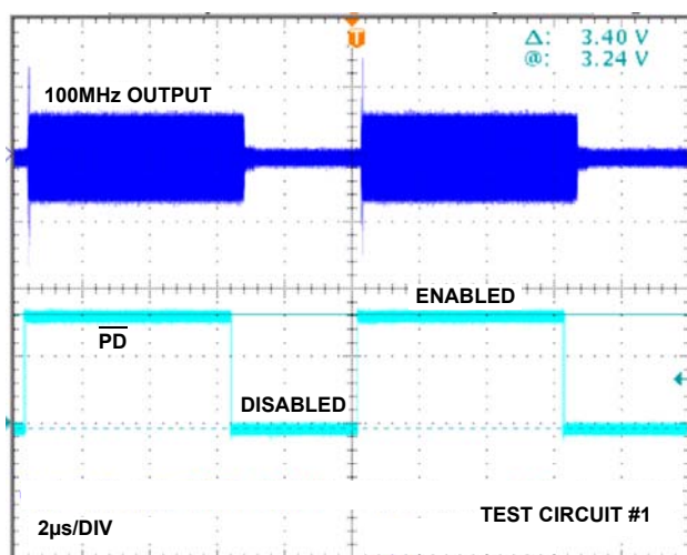
FIGURE 22. ENABLE/DISABLE TIMES
