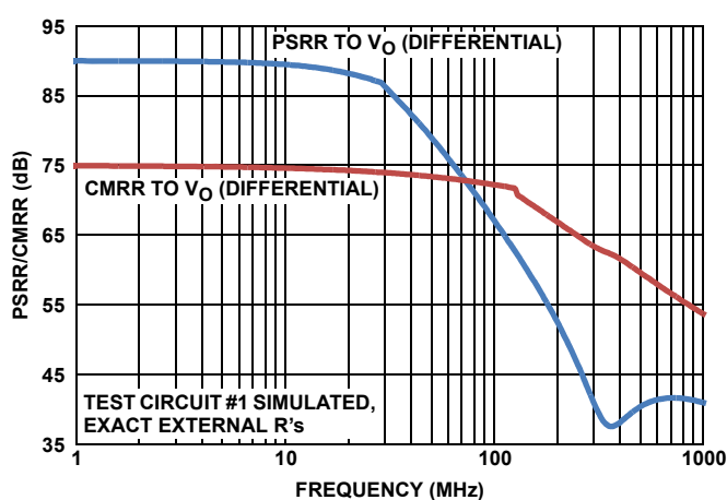
FIGURE 25. PSRR/CMRR TO DIFFERENTIAL V_O
