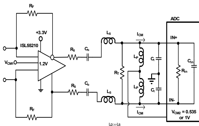
FIGURE 35. AC COUPLED, HIGHER FREQUENCY RLC FILTER DESIGN
