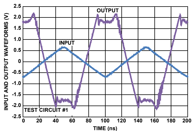
FIGURE 24. OVERDRIVE RECOVERY
