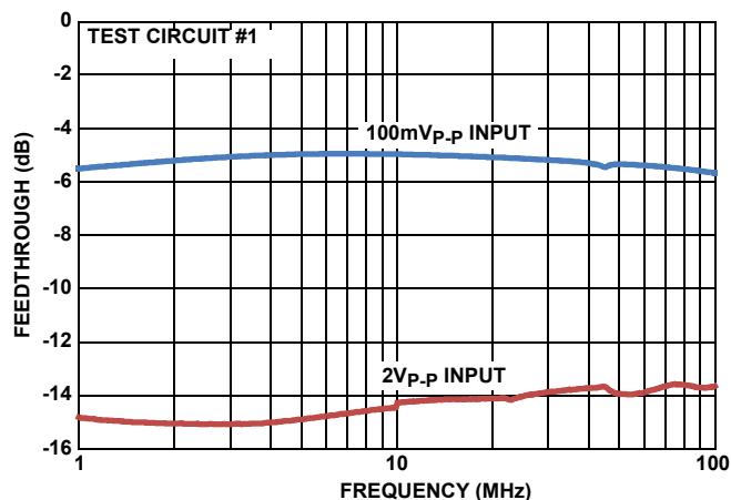
FIGURE 23. DISABLED FEEDTHROUGH
