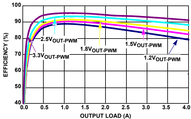
FIGURE 5. EFFICIENCY vs LOAD (1MHz 5V V_{IN} PWM)
