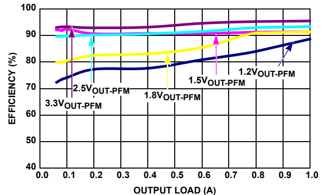
FIGURE 6. EFFICIENCY vs LOAD (1MHz 5V V_{IN} PFM)
