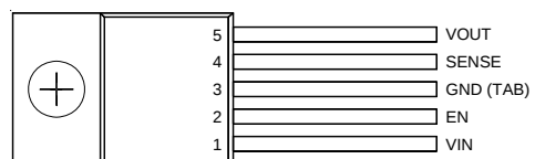
TO-220-5 RT9172S-□□xT5
