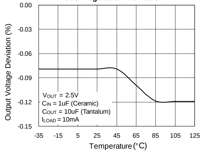
Load Regulation Deviation
