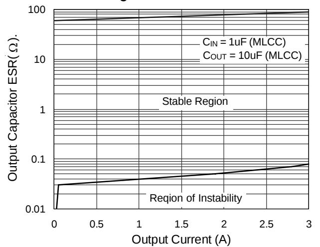
Range of Stable ESR Values
