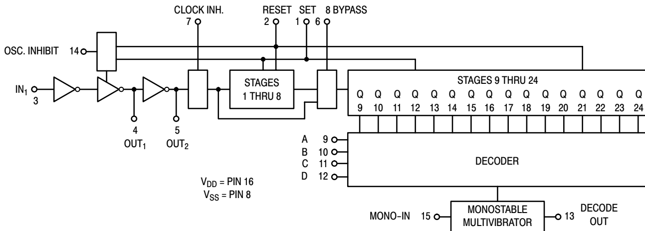
Figure 1. Block Diagram
