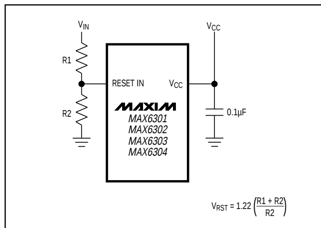
Figure 4. Monitoring a Voltage Other than V_{CC}
