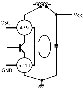
Fig.3 Oscillation loop
