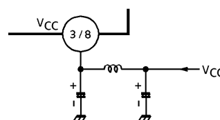
Fig.2 LC Filter
