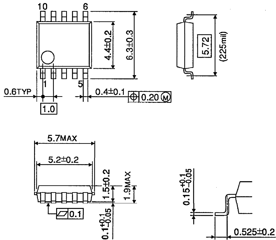
OUTLINE DRAWING SSOP10-P-225-1.00
