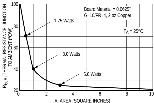
Figure 16. Thermal Resistance versus Drain Pad Area for the D 3 PAK Package (Typical)
