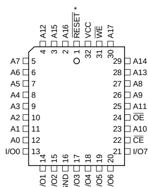
PLCC Top View
