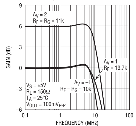
Frequency Response vs Closed Loop Gain ( I_S = 300\mu A per Amplifier)
