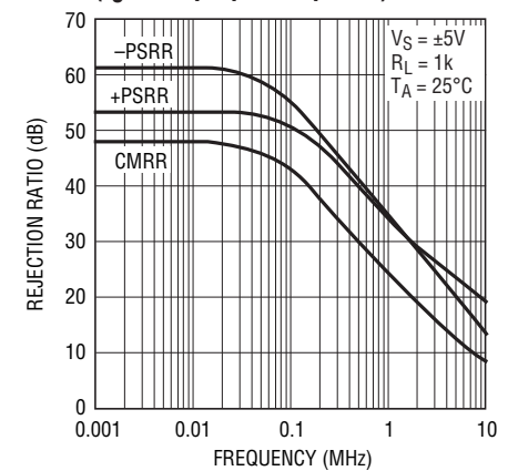
CMRR and PSRR vs Frequency ( I_S = 300\mu A per Amplifier)
