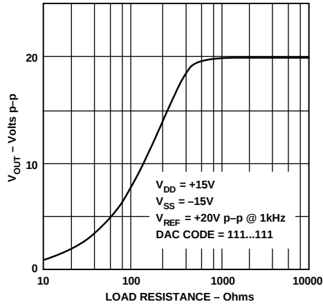
Output Voltage Swing vs. Resistive Load
