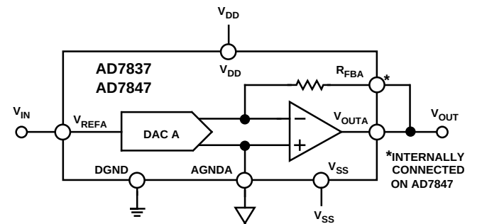
Figure 6. Unipolar Binary Operation
