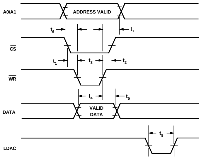
Figure 5. AD7837 Write Cycle Timing Diagram
