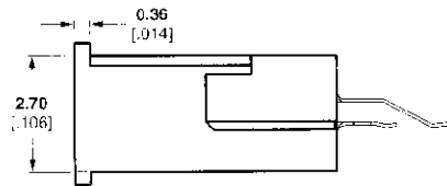
End View
