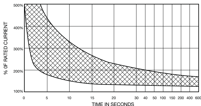
TIME vs. Percent of Rated Current Curves for 5-40 Amp. Circuit Breakers
