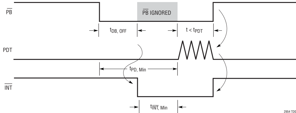
Off Interrupt Timing, \overline{\text{PB}} Pressed and Released, Enable Remains Active
