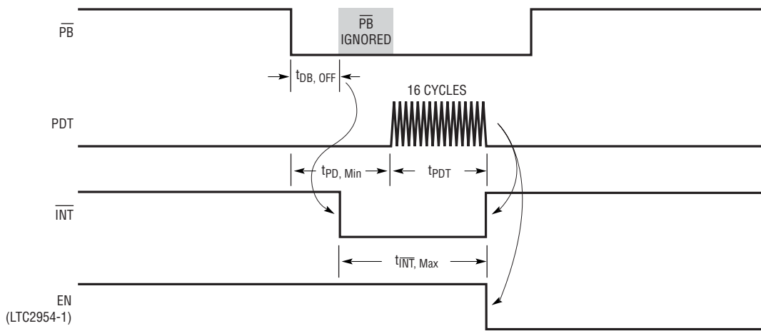
Forced Off, Power Down Timing, \overline{\text{PB}} Pressed and Held Low for t > (t_{\text{PD, Min}} + t_{\text{PDT}})
