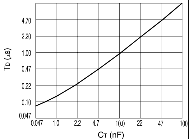
Deadtime vs C_T (3k R_T 100k)
