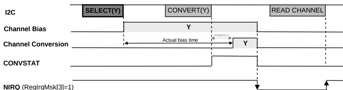
Figure 21 – Manual Mode – SELECT command (CHAN = Y; PROXSCANPERIOD = 0)
