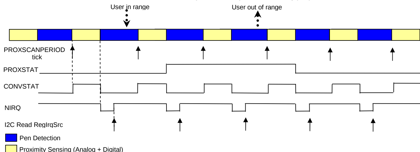
Figure 42 – Proximity Sensing Host Operation (Pen Trigger Mode ; ReglqMsk[6:4] = 010 ; PROXIRQSEL = 1)
