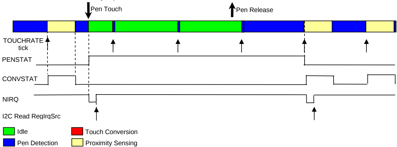
Figure 45 – Pen Detect Mode (RegIrqMsk[6:2] = 00011 ; PROXSCANPERIOD = 001 ie 1/TOUCHRATE)
