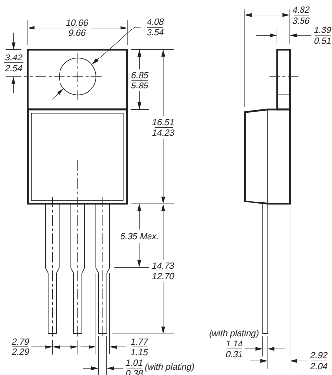
TO-220
