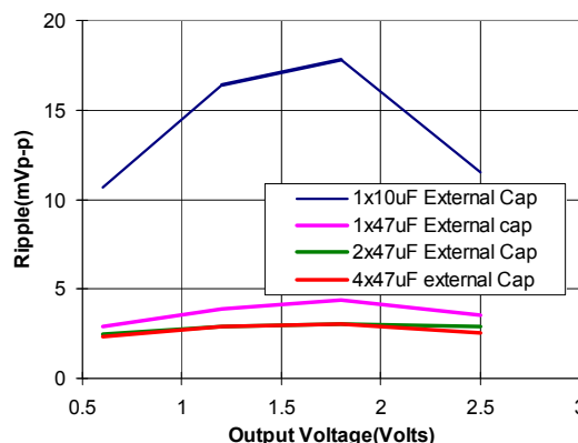
Figure 37. Output ripple voltage for various output voltages with external 1x10 \mu F, 1x47 \mu F, 2x47 \mu F or 4x47 \mu F ceramic capacitors at the output (3A load). Input voltage is 3.3V.
