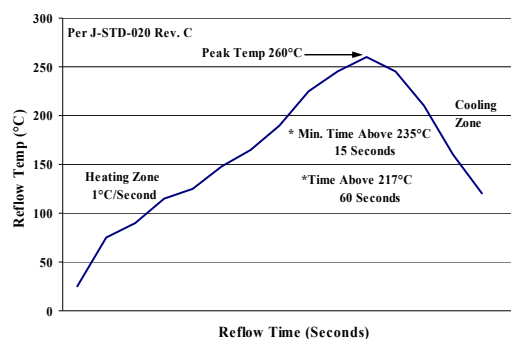
Figure 47. Recommended linear reflow profile using Sn/Ag/Cu solder.
