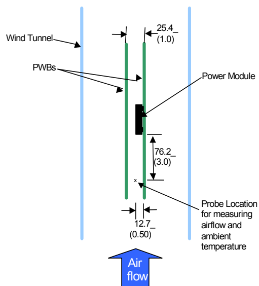
Figure 45. Thermal Test Setup.
