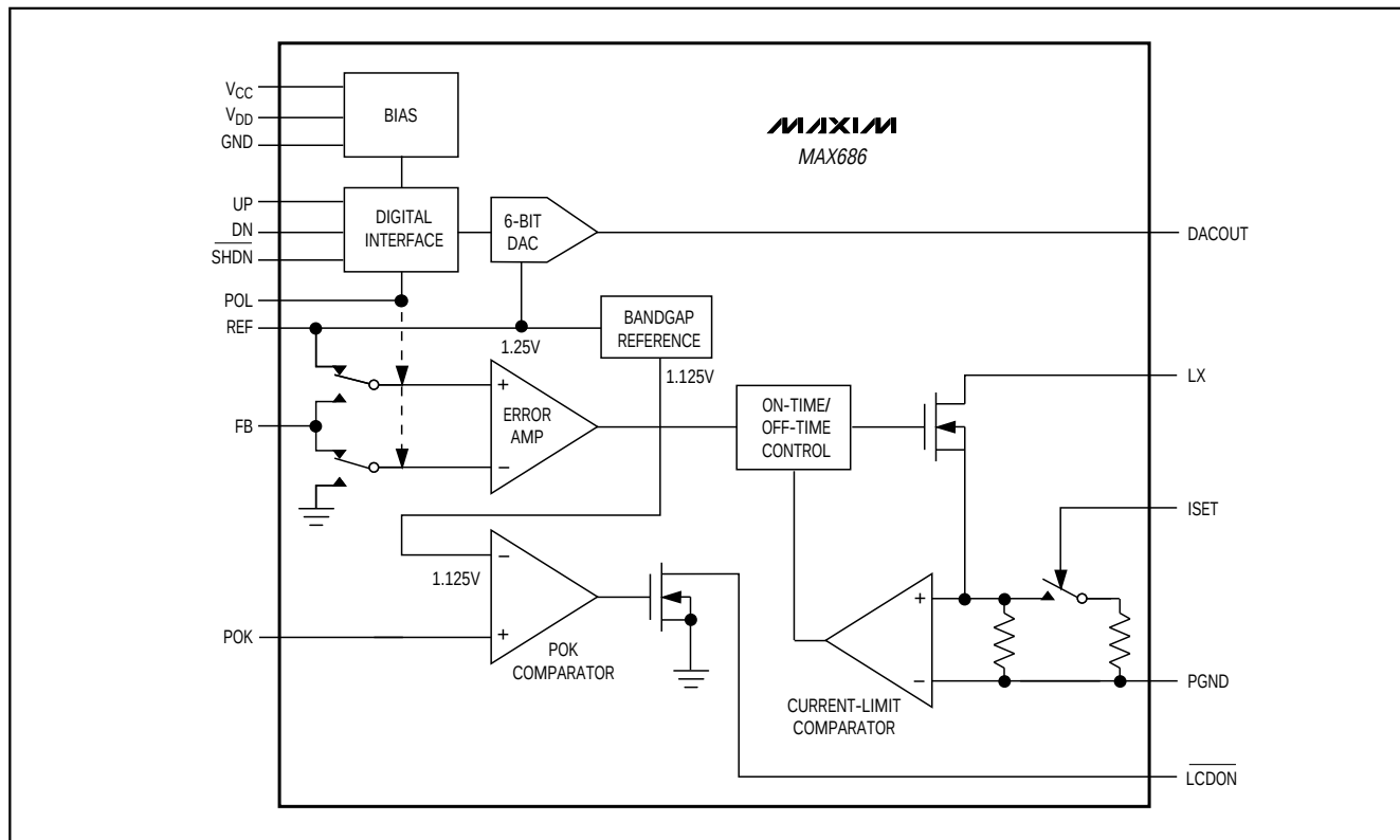
Functional Diagram
