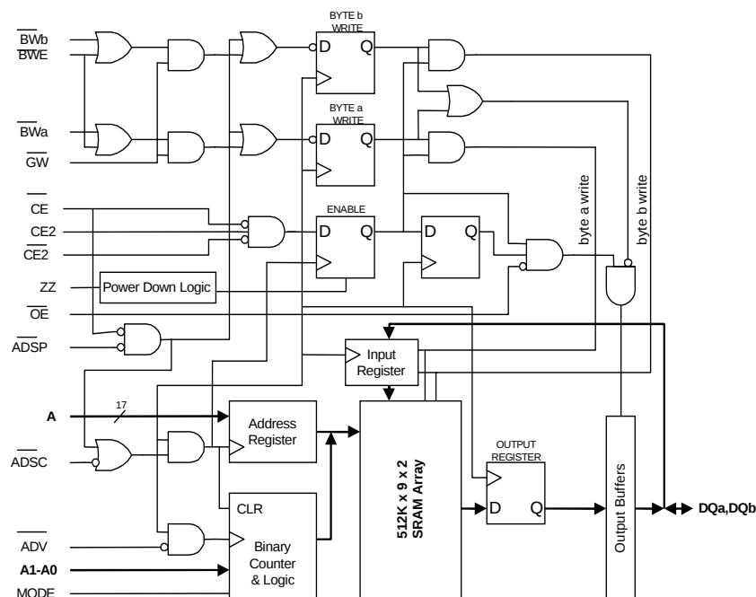
Functional Block Diagram—512K × 18 [1]
