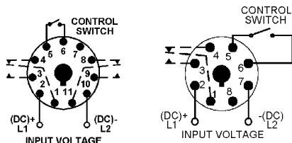
11 Pin DPDT
