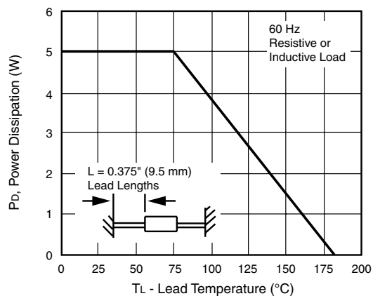
Figure 4. Power Derating Curve
