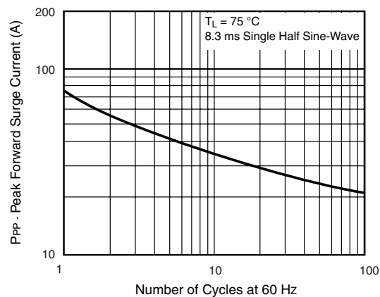
Figure 5. Maximum Non-Repetitive Forward Surge Current
