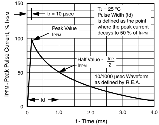
Figure 2. Pulse Waveform
