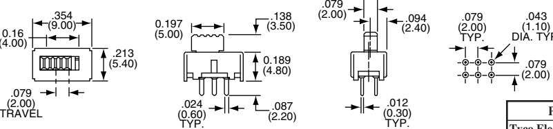
SSB22
