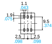
Recommended PC board pattern (TOP VIEW 2:1)
