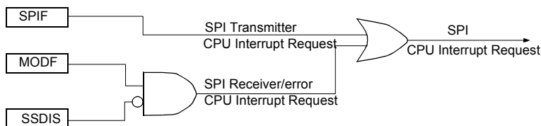
Figure 88. SPI Interrupt Requests Generation
