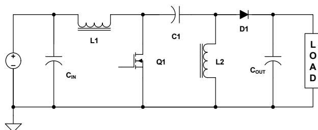
FIGURE 12. SEPIC TOPOLOGY
