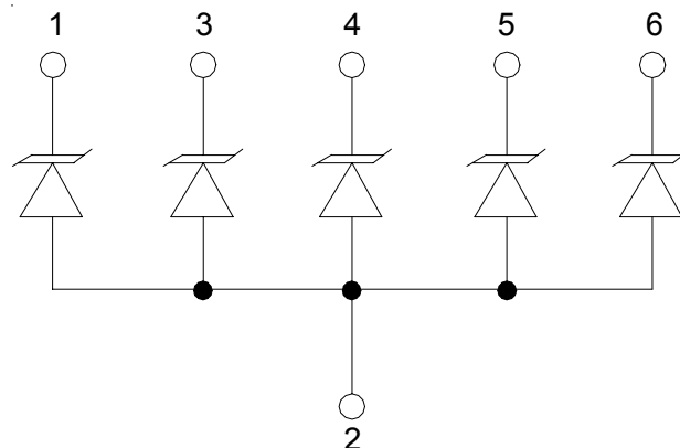
Protection of Five Unidirectional Lines
