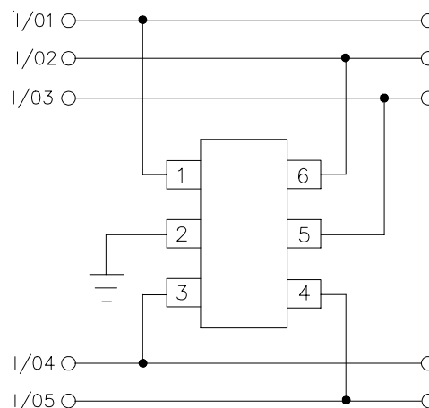
Protection of Five Unidirectional Lines
